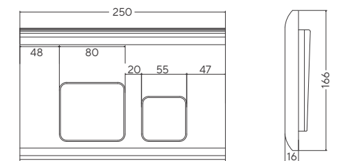
Q507455120 Sisma Flush Plate MRP: ₹ 1,790
