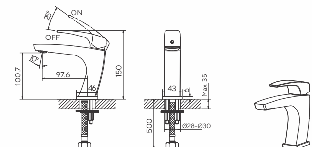
Q253112120 Pillar Cock "MARSALA" MRP: ₹ 10,990
