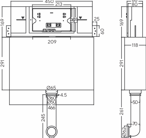
Concealed Cistern Sisma with Half Frame - QF
