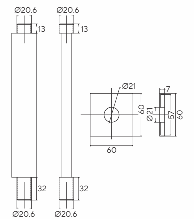
Q503151120 Square Shower Arm Ceiling 250mm Polished Chrome MRP: ₹ 3,490
