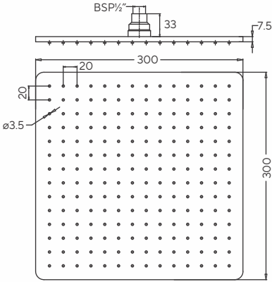
Q503146220 Overhead Shower 300x300mm in Chrome MRP: ₹ 14,990
