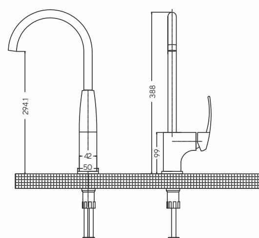
Q253118120 Marsala Single Function Deck-Mount Kitchen Faucet MRP: ₹ 12,990
